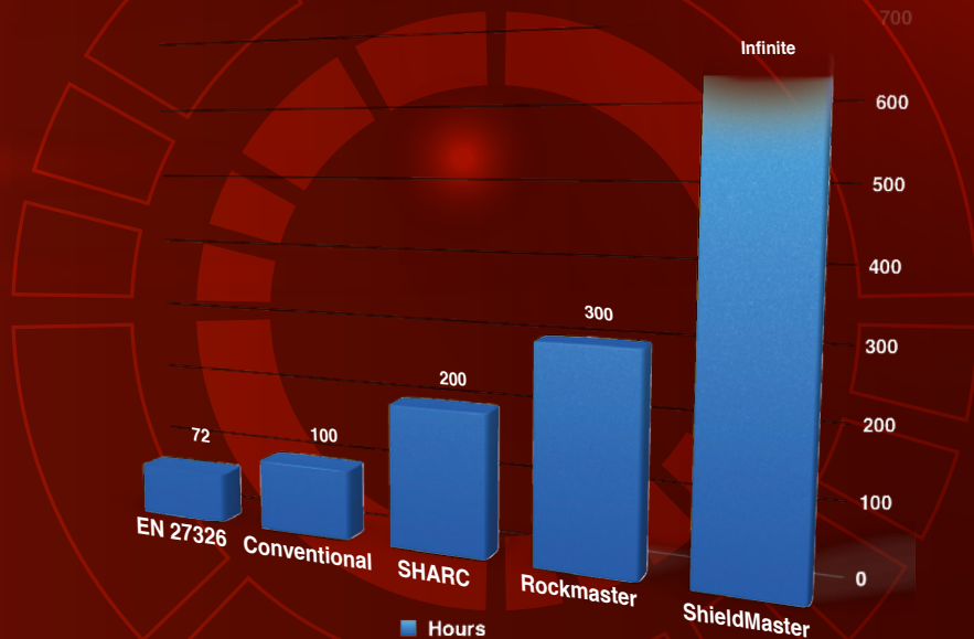
Ozone Resistance 2
