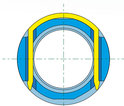
Cross-section of a Flushfit fitting with staple in-situ
